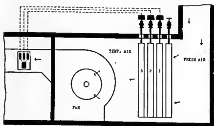
FIG. 4. DIAGRAM SHOWING APPLICATION OF A MULTIPLE THERMOSTAT TO HOT-BLAST HEATING
